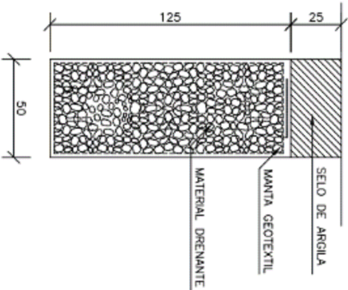
DPS 05 (DRENO CEGO)
